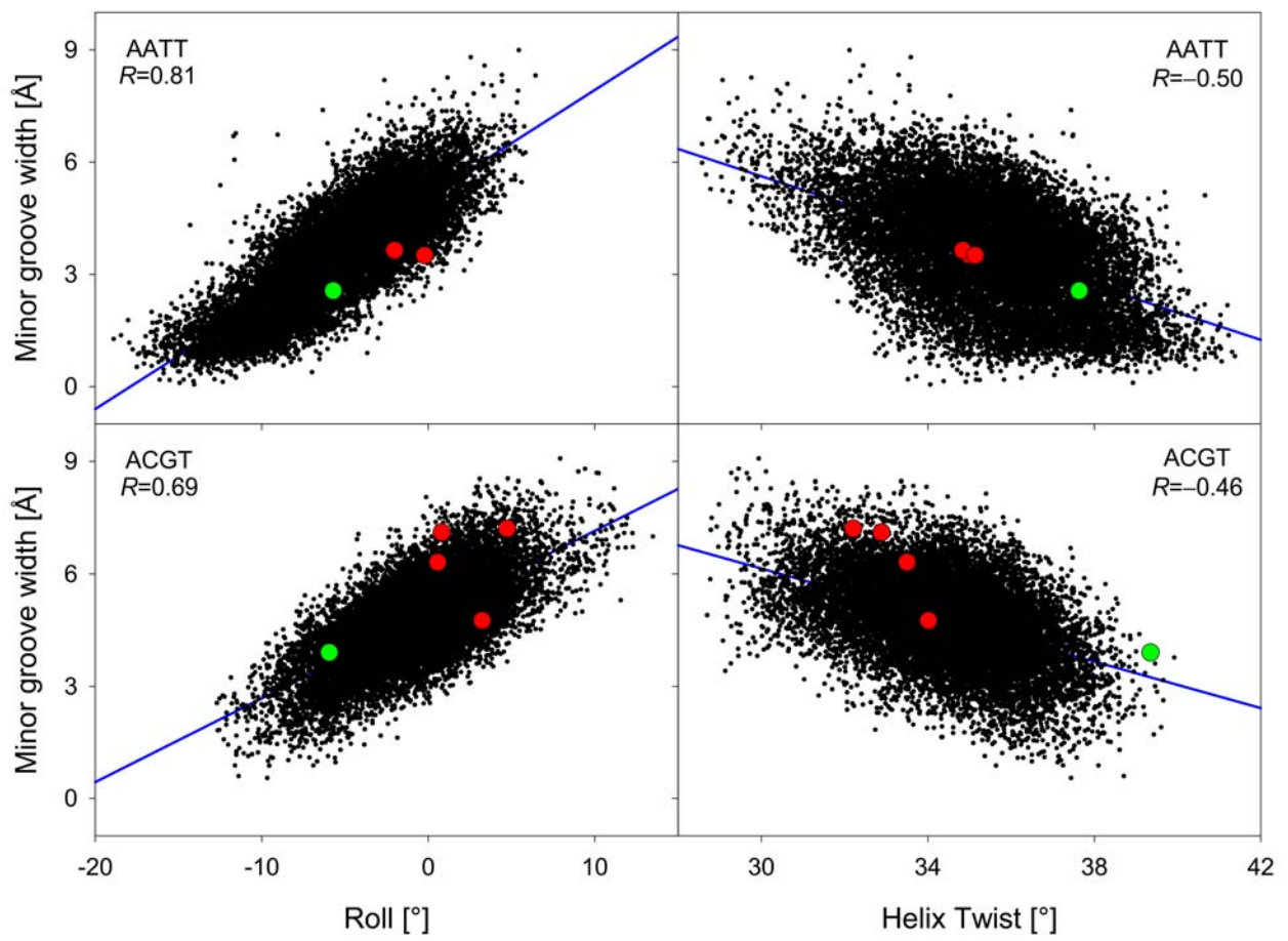
Rohs et al. (2005) Structure 13, 1505 Figure 5.
