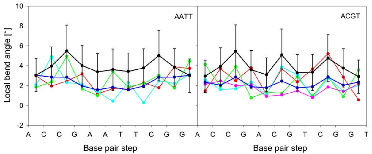
Rohs et al. (2005) Structure 13, 1505 Figure 6.
