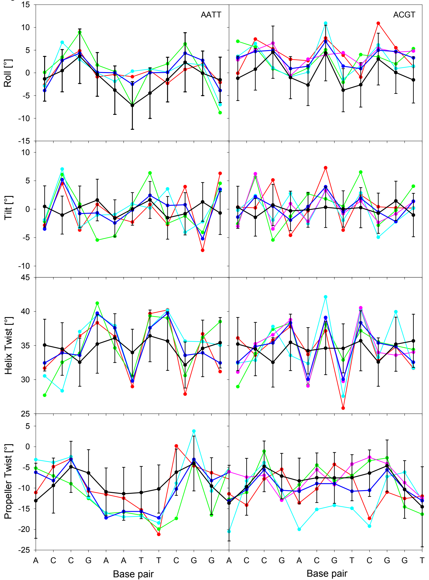
Rohs et al. (2005) Structure 13, 1504 Figure 4.
